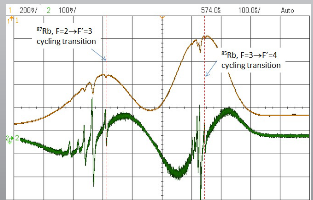
Doppler-broadened and Doppler-free spectra of D2 hyperfine transitions of Rb
